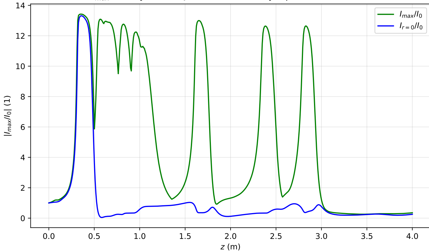
I_{max}(x=0, y=0, z)/I_0 , \text{Pin}=8.3\text{Pcr} , noisy input, artificial time
